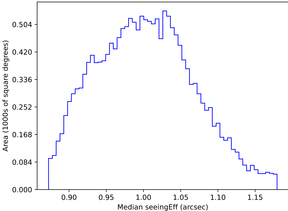
too_elab_r256_d2_gz_v3.4_10yrs WFD z band: Median seeingEff
