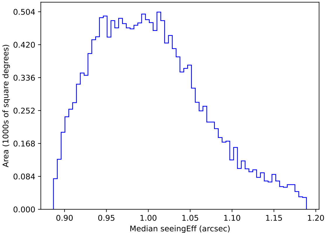
too_elab_r256_d2_gz_v3.4_10yrs WFD y band: Median seeingEff
