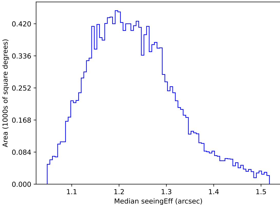
too_elab_r256_d2_gz_v3.4_10yrs WFD u band: Median seeingEff
