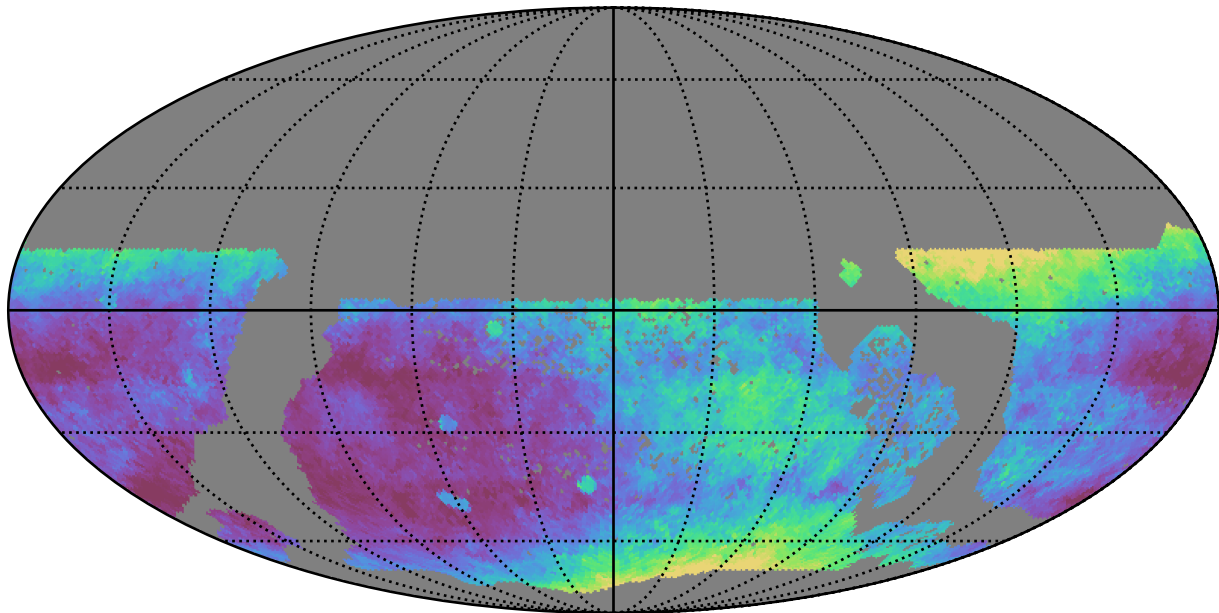
too_elab_r256_d2_gz_v3.4_10yrs WFD r band: Median seeingEff
