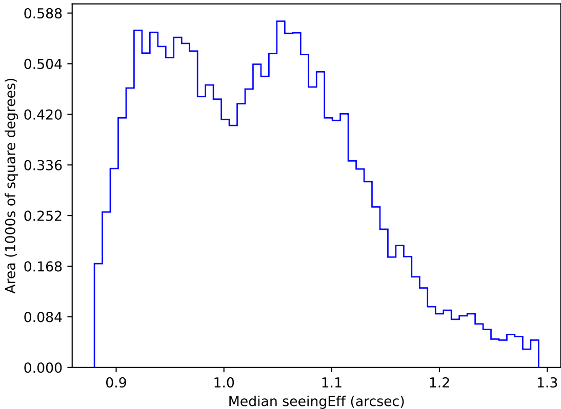
too_elab_r256_d2_gz_v3.4_10yrs WFD r band: Median seeingEff
