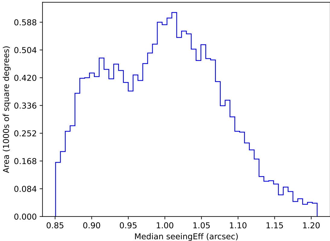
too_elab_r256_d2_gz_v3.4_10yrs WFD i band: Median seeingEff
