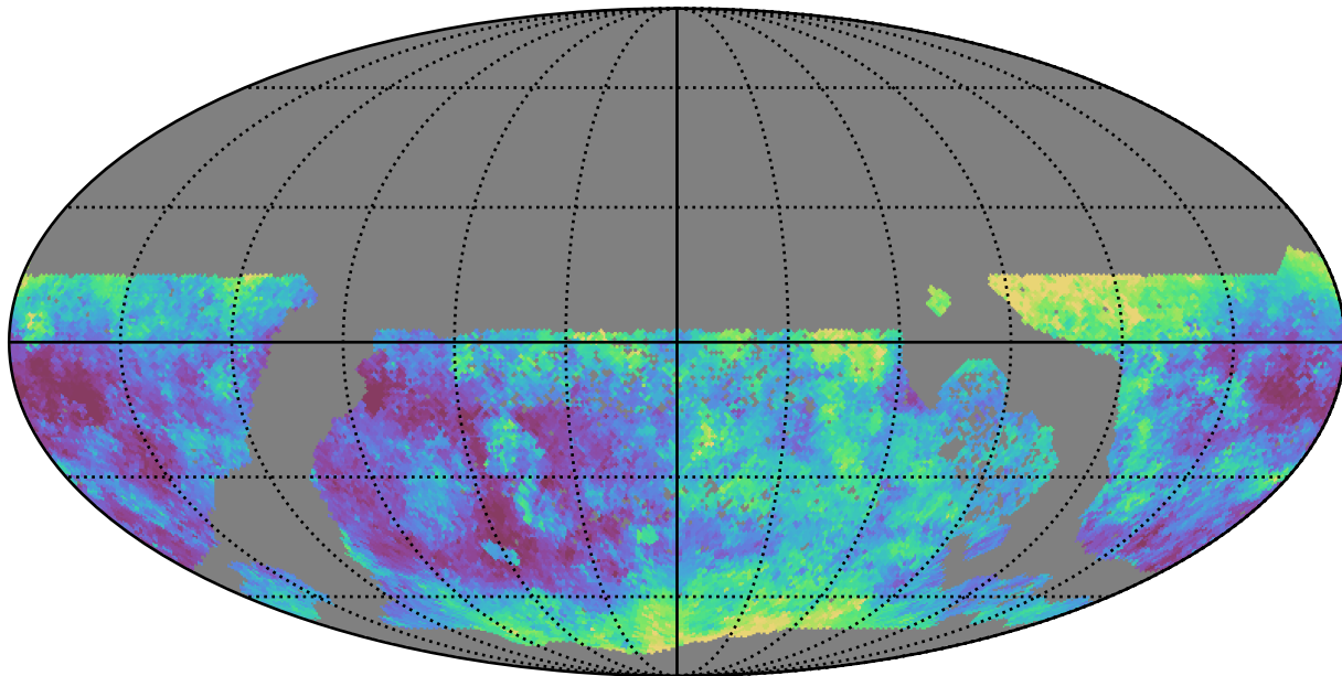
too_elab_r256_d2_gz_v3.4_10yrs WFD g band: Median seeingEff
