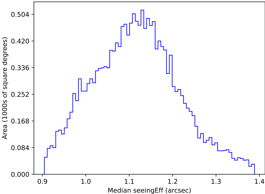
too_elab_r256_d2_gz_v3.4_10yrs WFD g band: Median seeingEff
