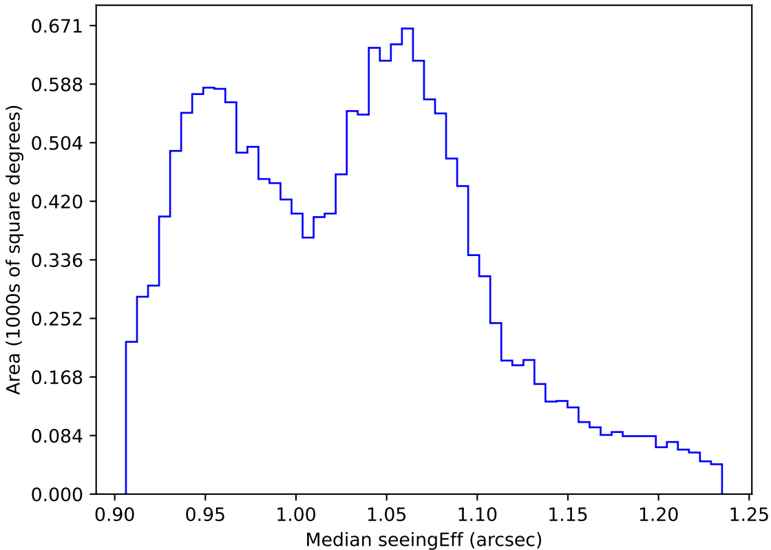
too_elab_r256_d2_gz_v3.4_10yrs WFD all bands: Median seeingEff
