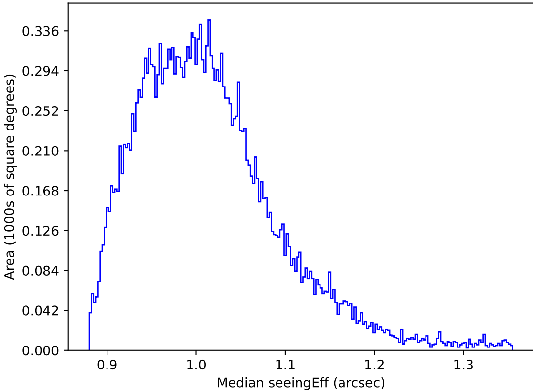
too_elab_r256_d2_gz_v3.4_10yrs All sky y band: Median seeingEff
