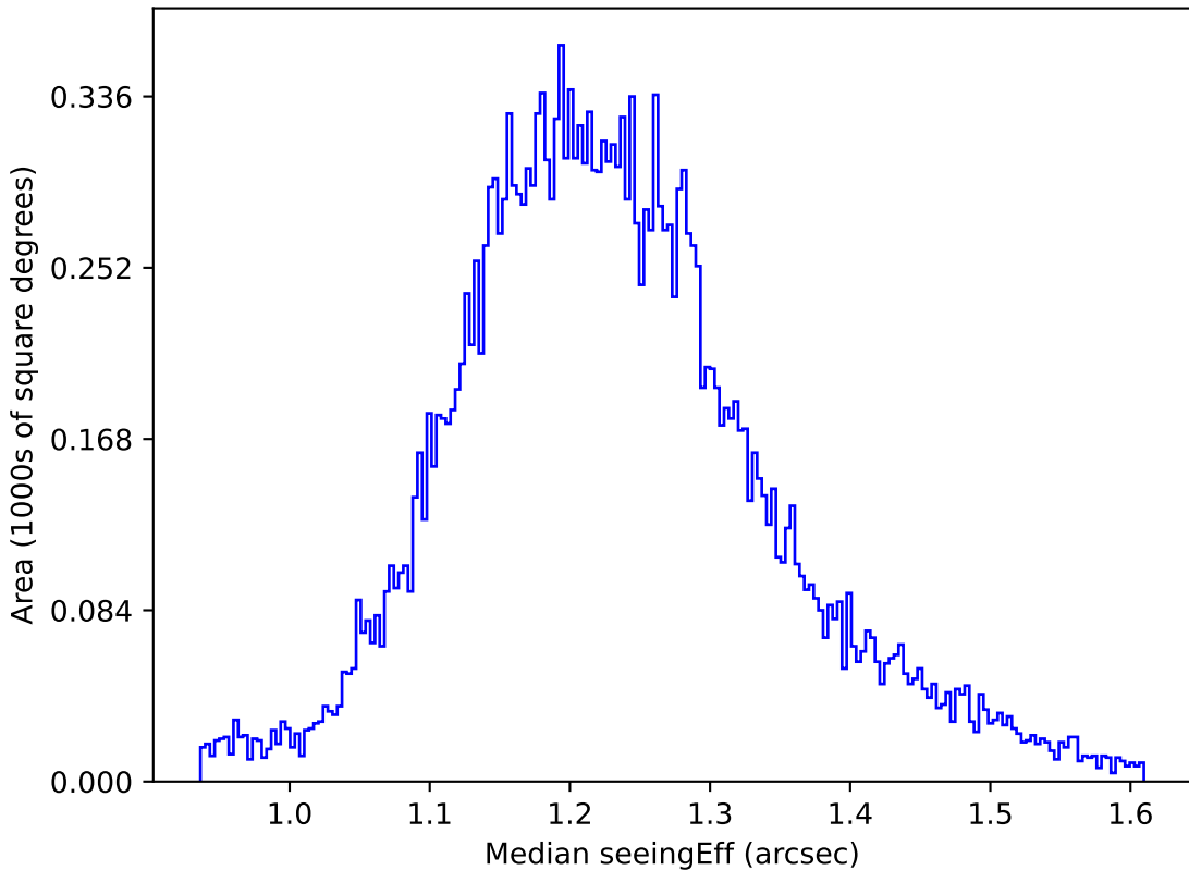
too_elab_r256_d2_gz_v3.4_10yrs All sky u band: Median seeingEff
