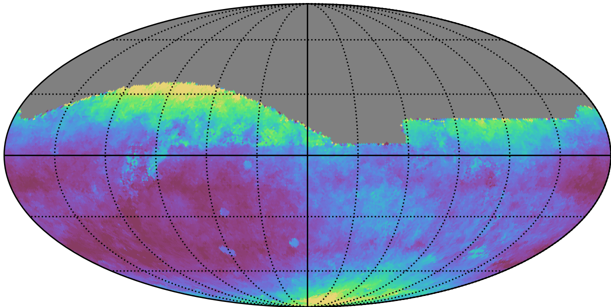
too_elab_r256_d2_gz_v3.4_10yrs All sky r band: Median seeingEff
