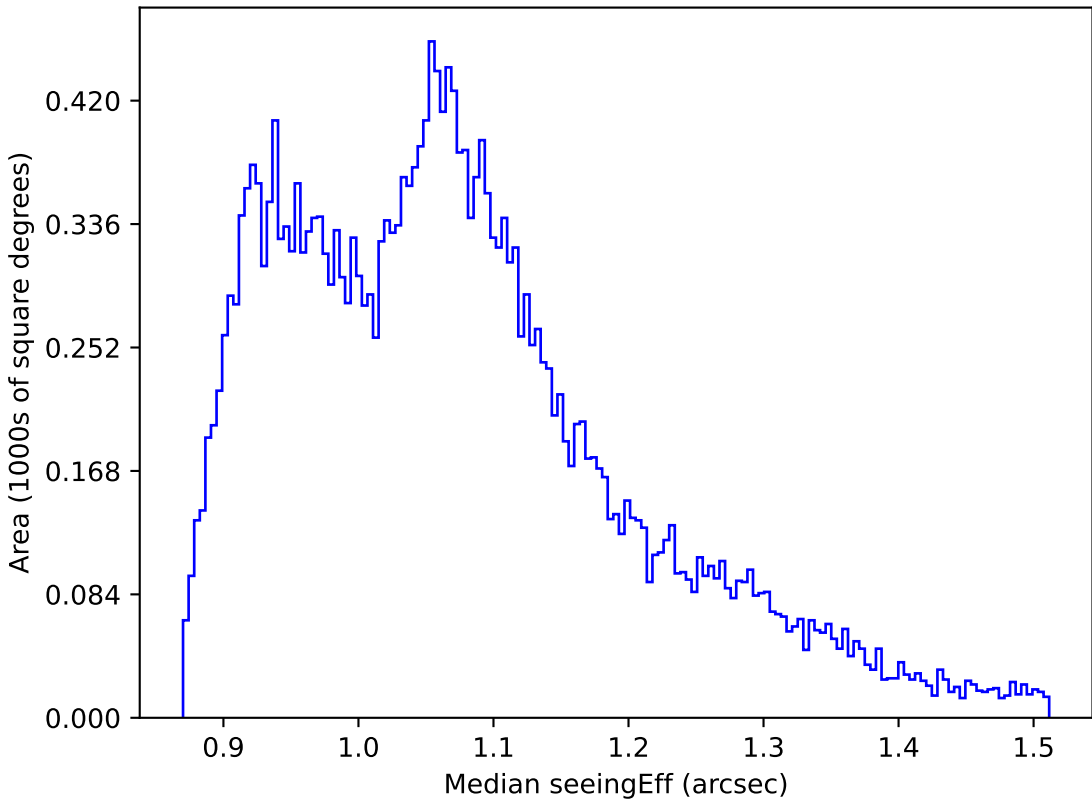
too_elab_r256_d2_gz_v3.4_10yrs All sky r band: Median seeingEff
