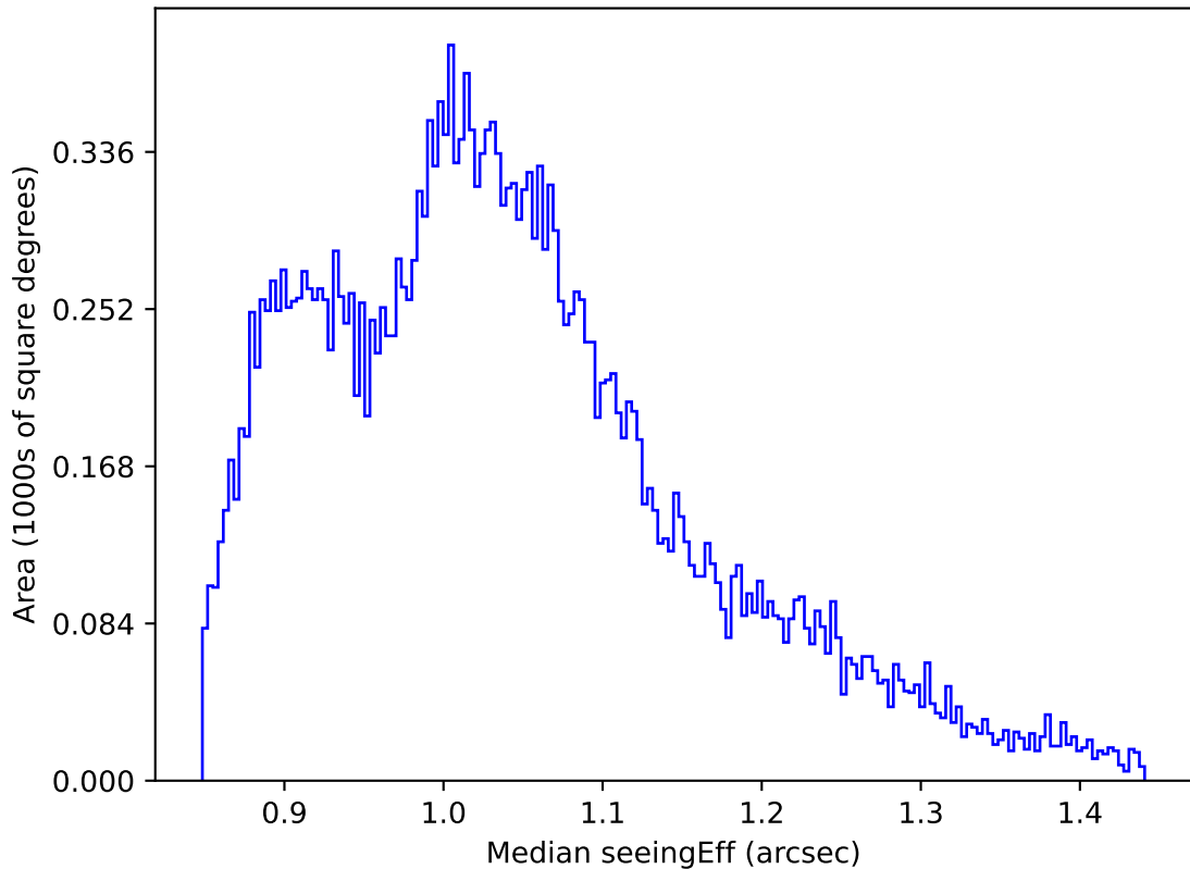
too_elab_r256_d2_gz_v3.4_10yrs All sky i band: Median seeingEff
