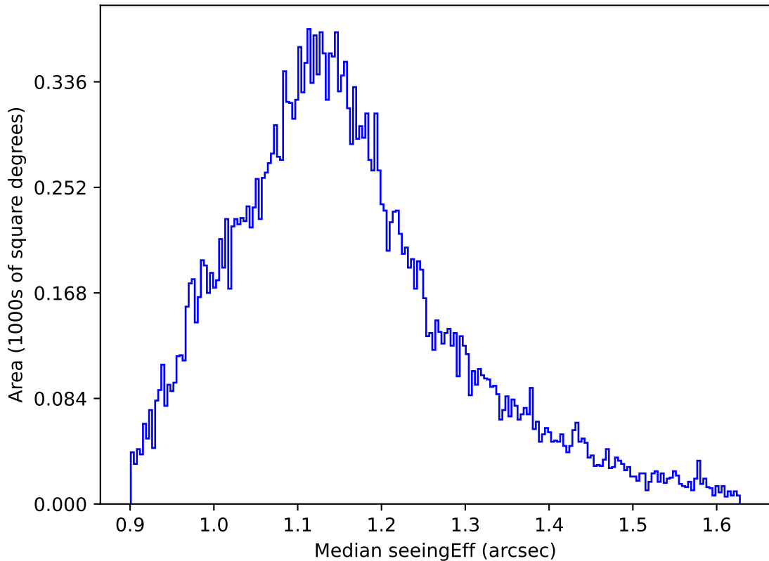
too_elab_r256_d2_gz_v3.4_10yrs All sky g band: Median seeingEff
