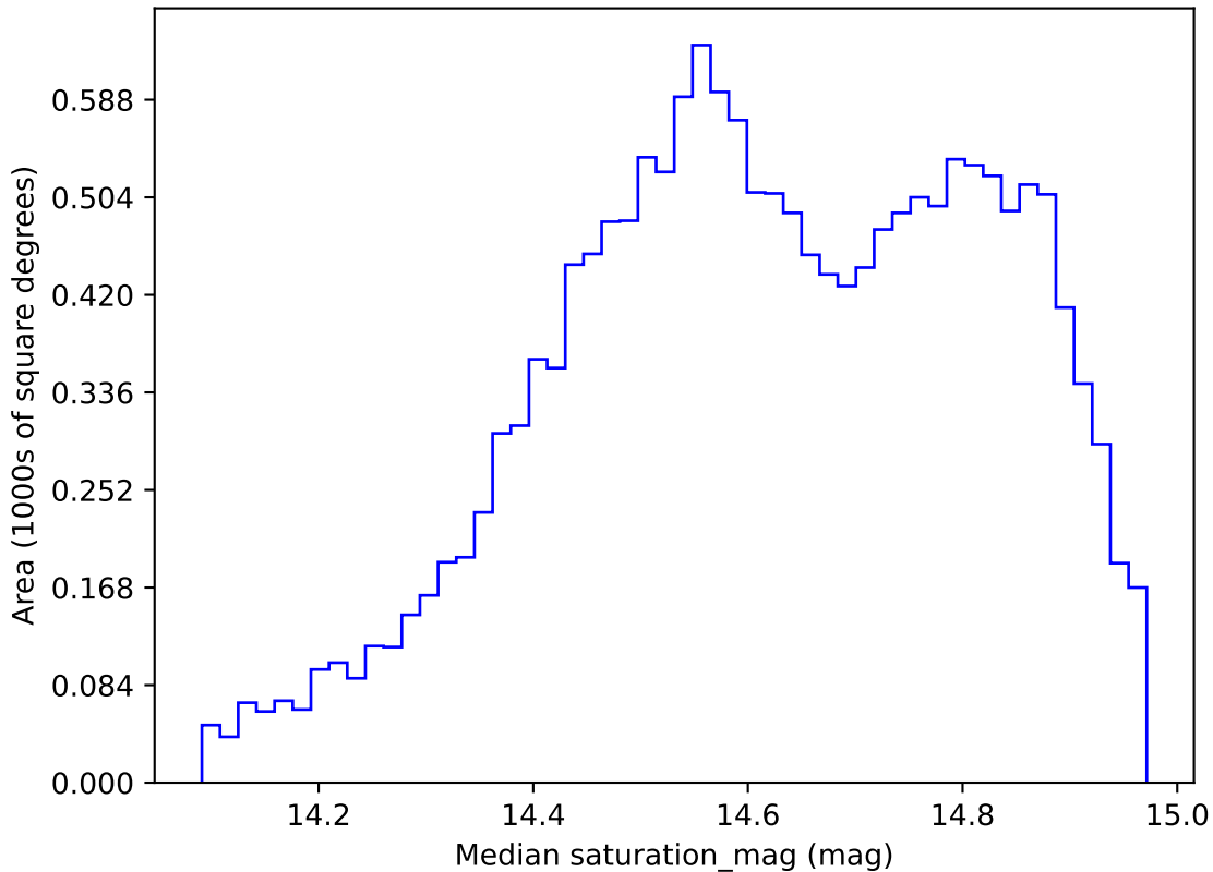
too_elab_r256_d2_gz_v3.4_10yrs WFD r band: Median saturation_mag
