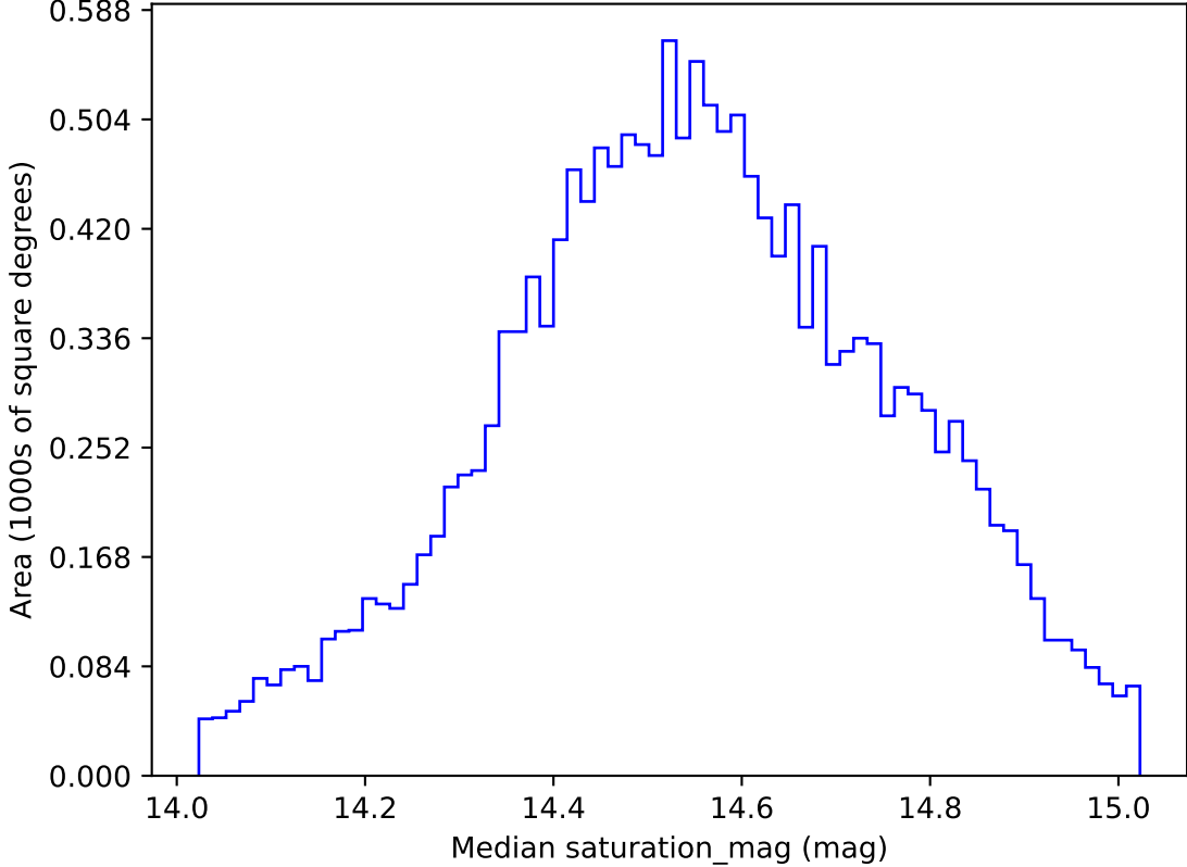
too_elab_r256_d2_gz_v3.4_10yrs WFD g band: Median saturation_mag
