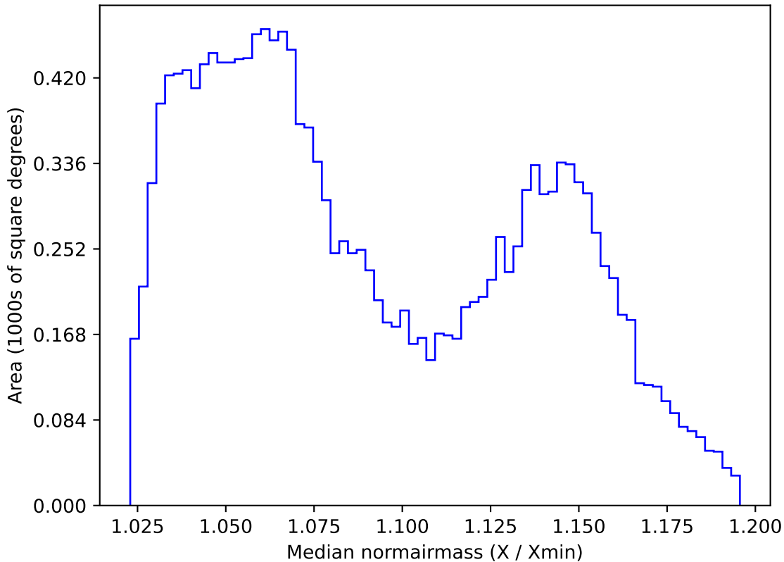
too_elab_r256_d2_gz_v3.4_10yrs WFD z band: Median normairmass
