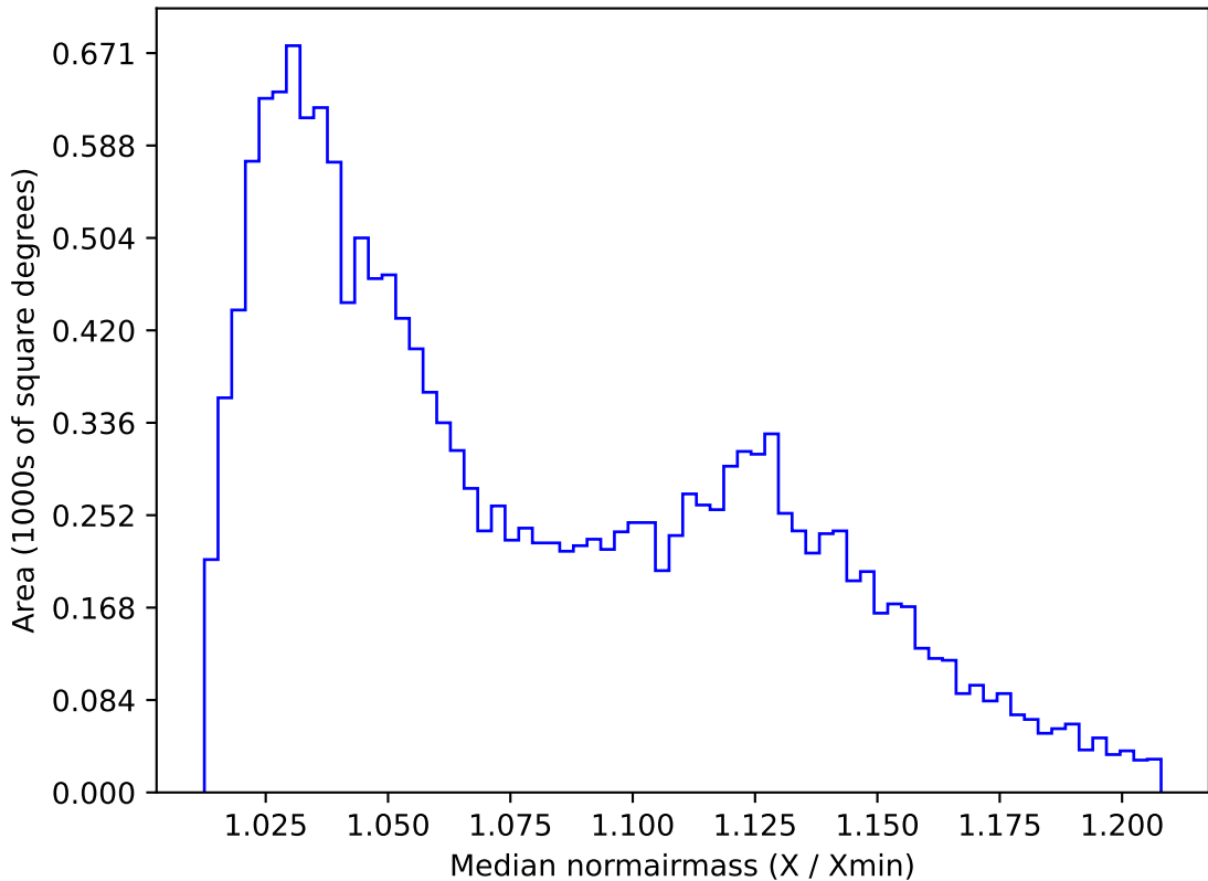
too_elab_r256_d2_gz_v3.4_10yrs WFD u band: Median normairmass
