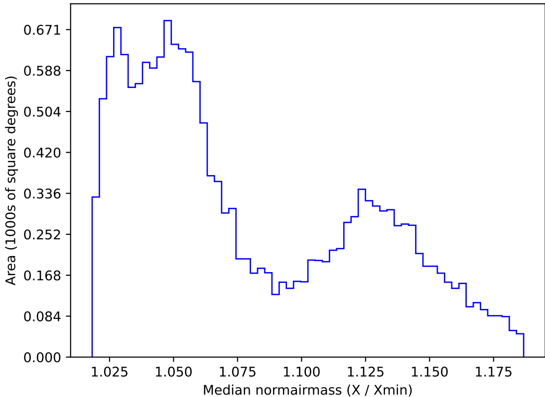
too_elab_r256_d2_gz_v3.4_10yrs WFD r band: Median normairmass
