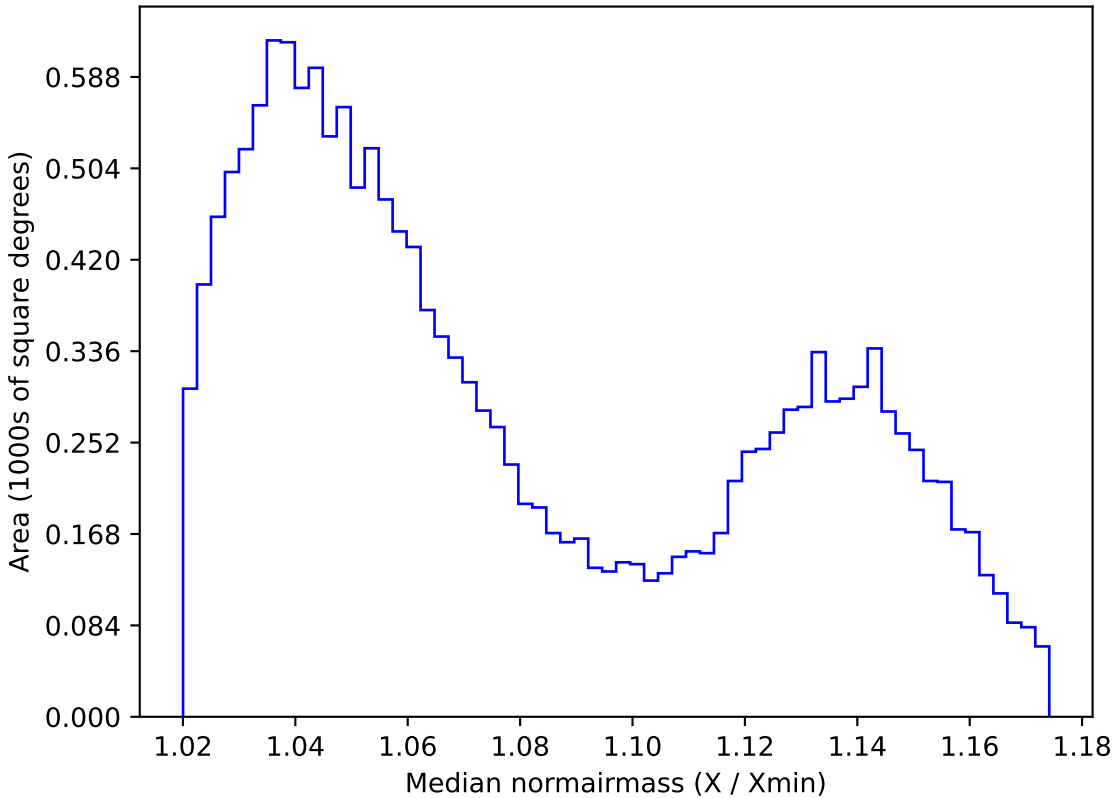
too_elab_r256_d2_gz_v3.4_10yrs WFD i band: Median normairmass
