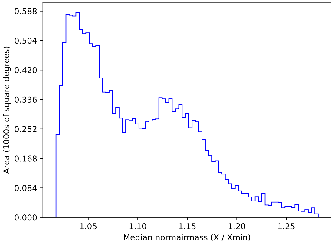
too_elab_r256_d2_gz_v3.4_10yrs WFD g band: Median normairmass
