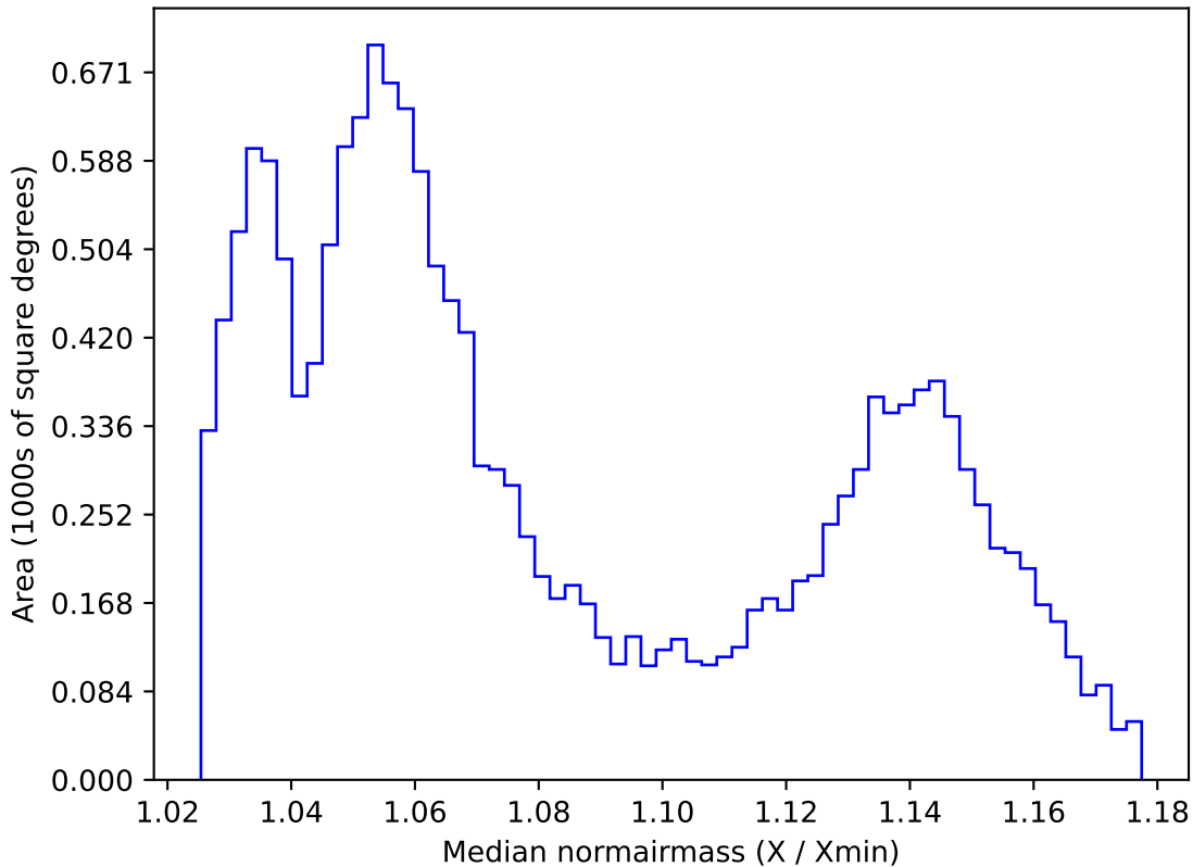
too_elab_r256_d2_gz_v3.4_10yrs WFD all bands: Median normairmass
