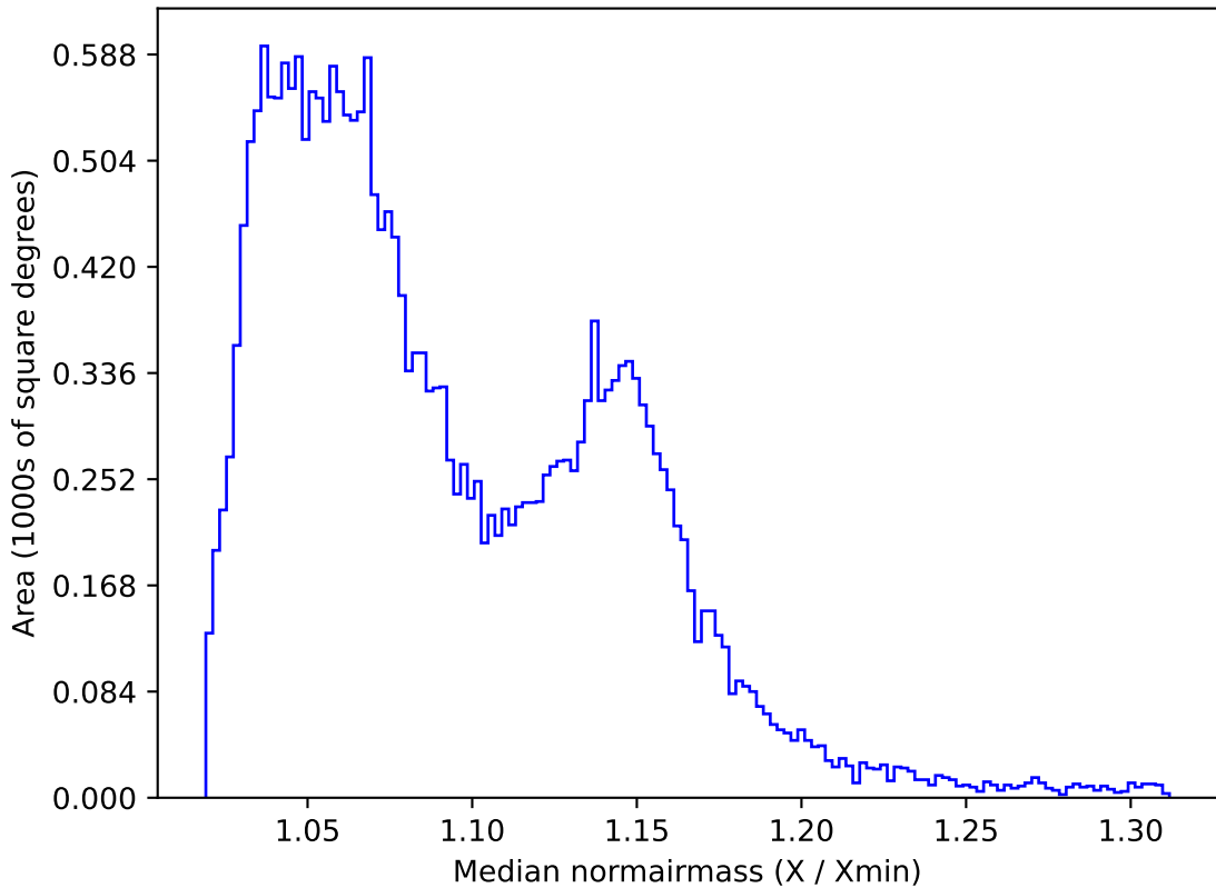
too_elab_r256_d2_gz_v3.4_10yrs All sky z band: Median normairmass
