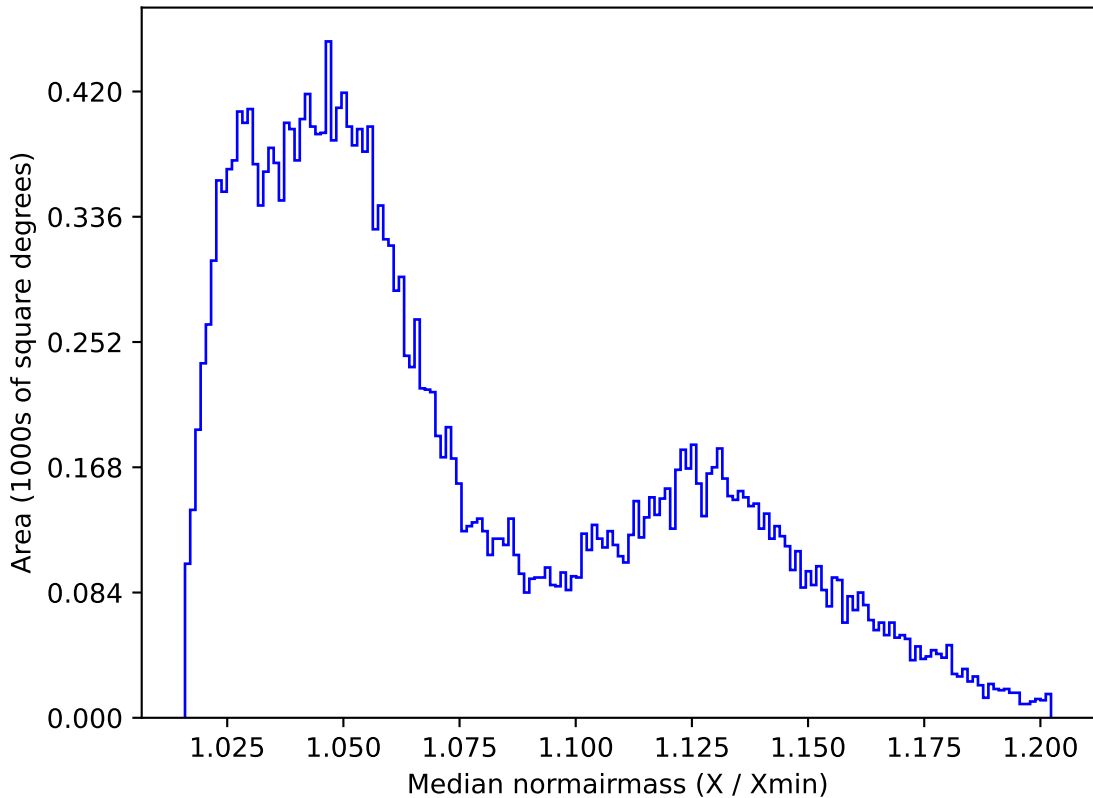
too_elab_r256_d2_gz_v3.4_10yrs All sky r band: Median normairmass
