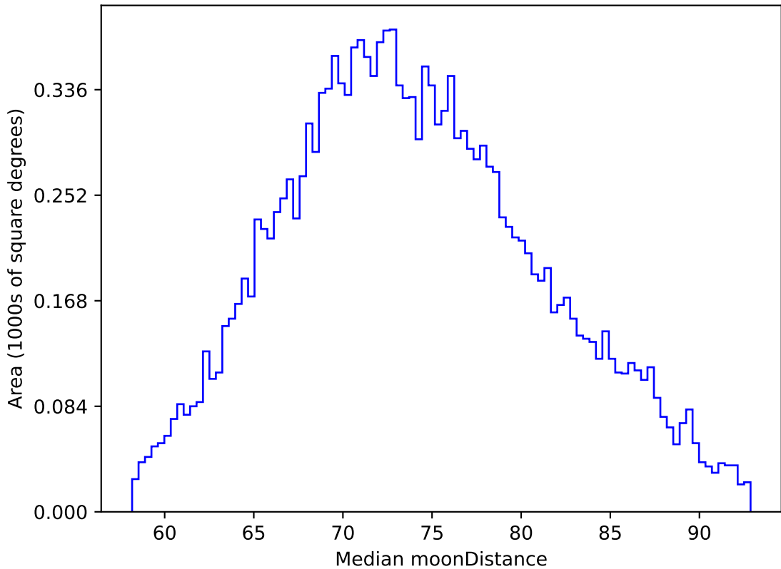
too_elab_r256_d2_gz_v3.4_10yrs WFD z band: Median moonDistance
