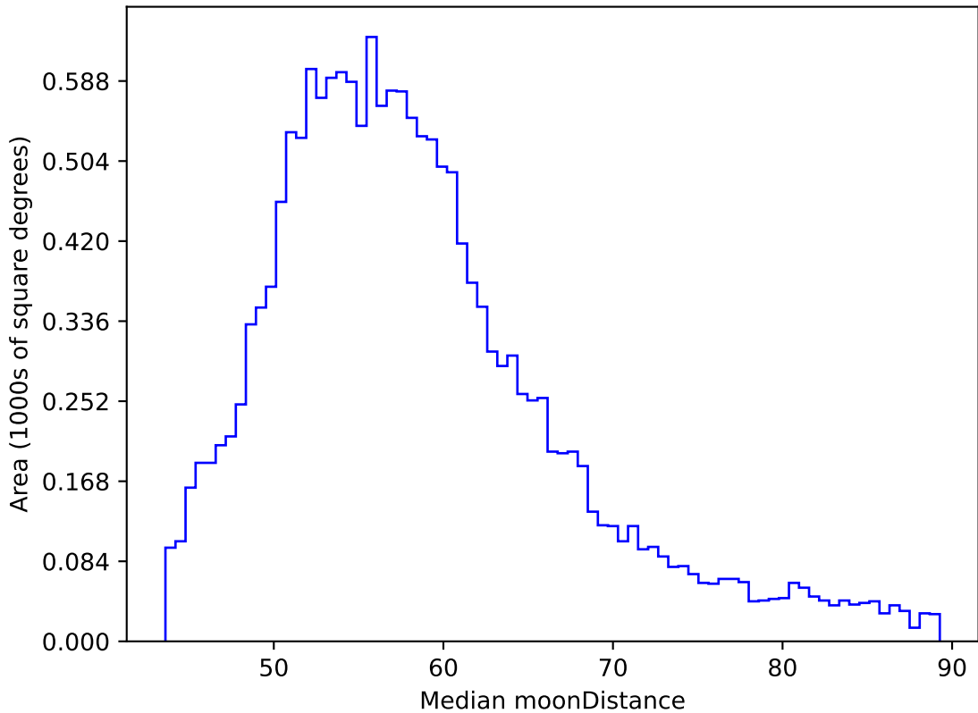
too_elab_r256_d2_gz_v3.4_10yrs WFD y band: Median moonDistance
