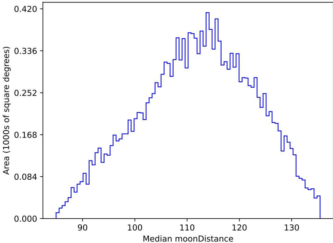
too_elab_r256_d2_gz_v3.4_10yrs WFD g band: Median moonDistance
