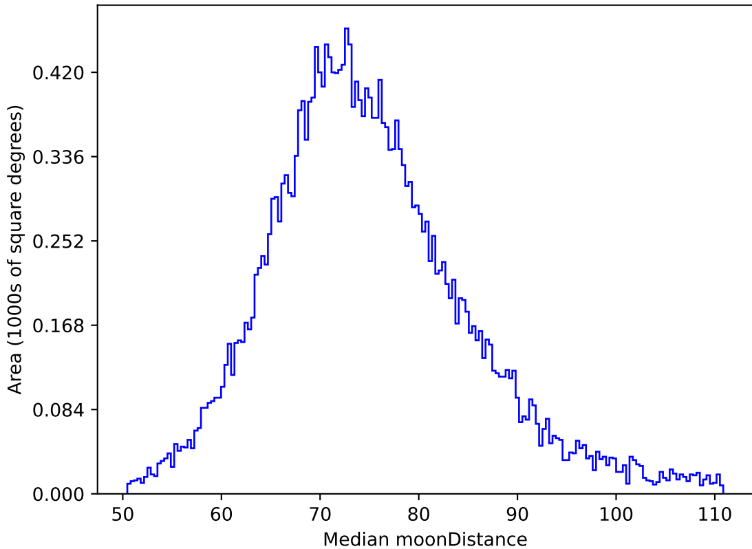
too_elab_r256_d2_gz_v3.4_10yrs All sky z band: Median moonDistance
