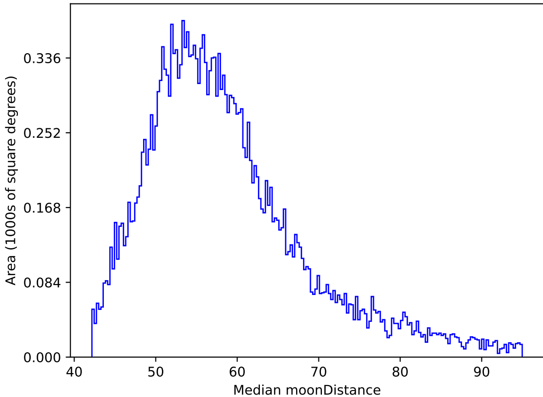
too_elab_r256_d2_gz_v3.4_10yrs All sky y band: Median moonDistance
