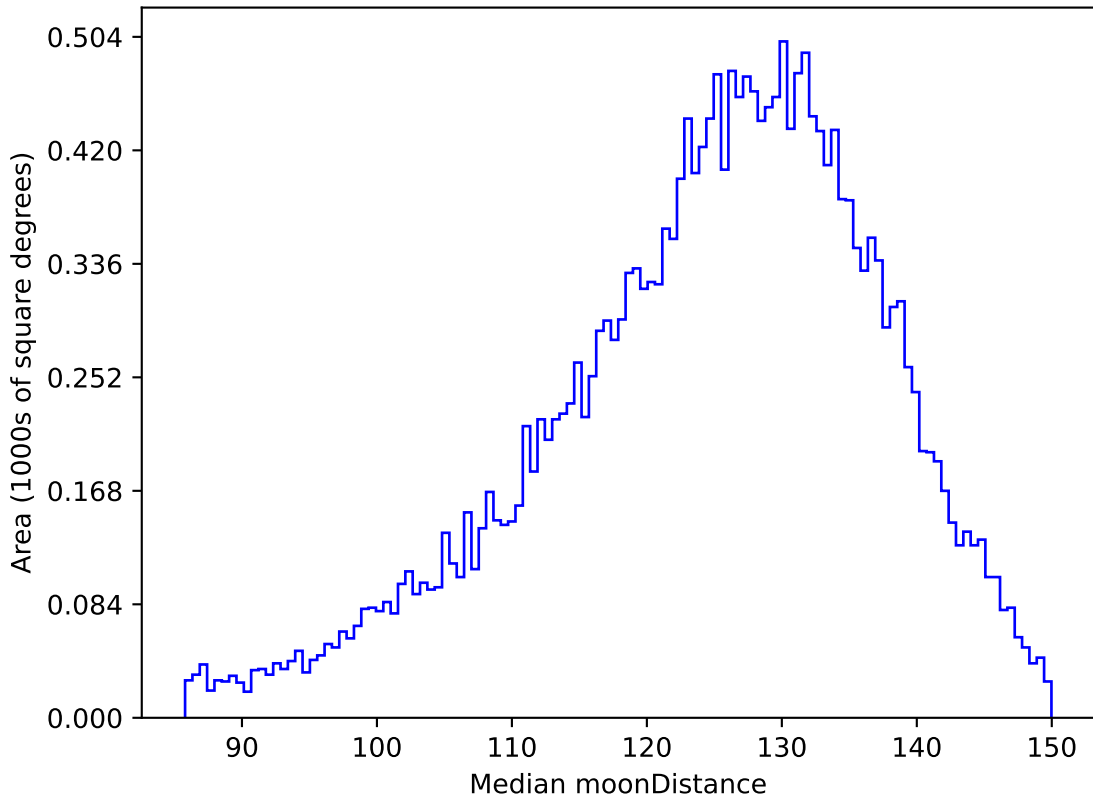
too_elab_r256_d2_gz_v3.4_10yrs All sky u band: Median moonDistance
