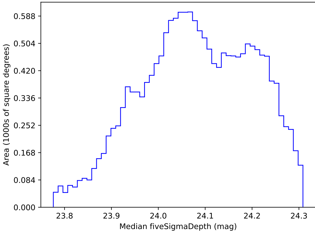
too_elab_r256_d2_gz_v3.4_10yrs WFD r band: Median fiveSigmaDepth
