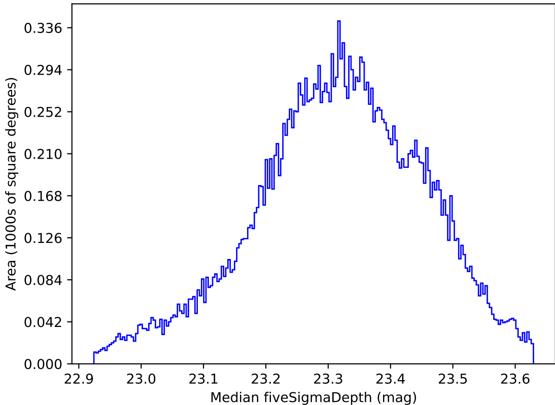
too_elab_r256_d2_gz_v3.4_10yrs All sky all bands: Median fiveSigmaDepth
