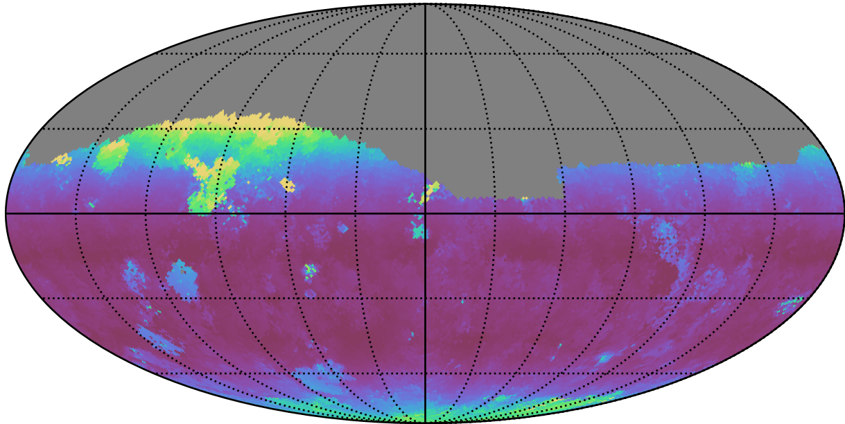
too_elab_r256_d2_gz_v3.4_10yrs Yr 1 z band: Median airmass
