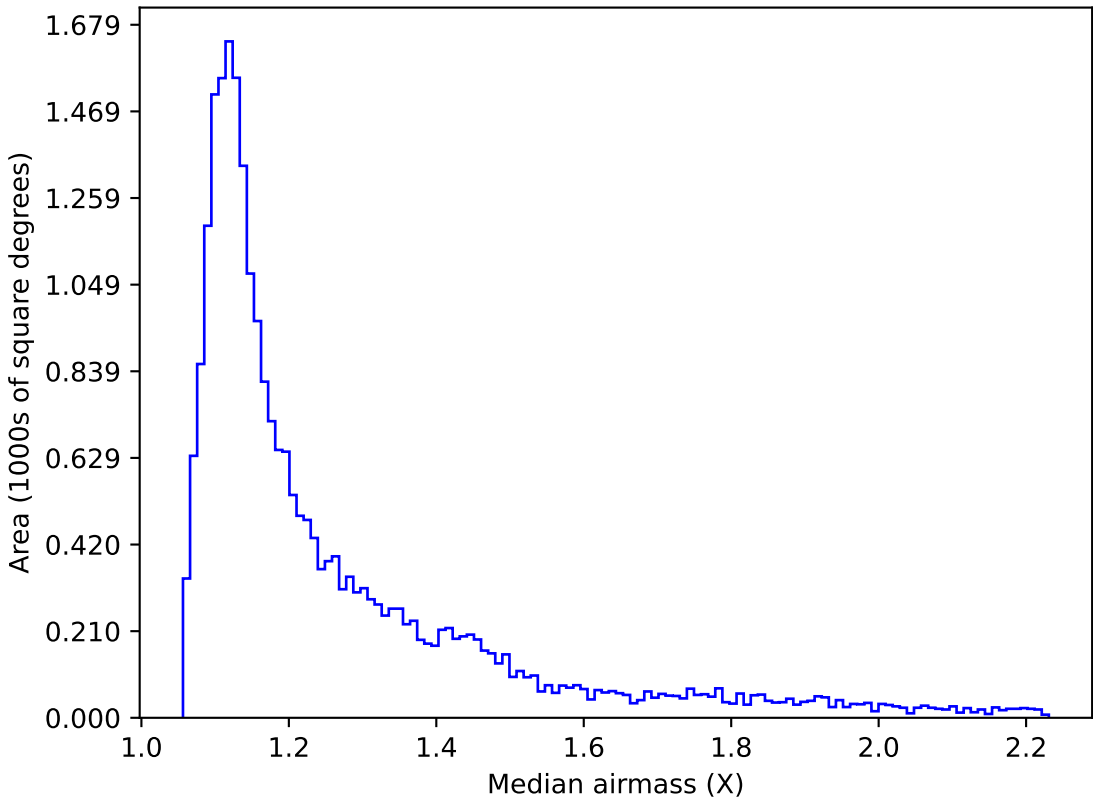
too_elab_r256_d2_gz_v3.4_10yrs Yr 1 z band: Median airmass
