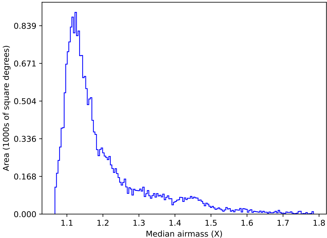
too_elab_r256_d2_gz_v3.4_10yrs Yr 1 y band: Median airmass
