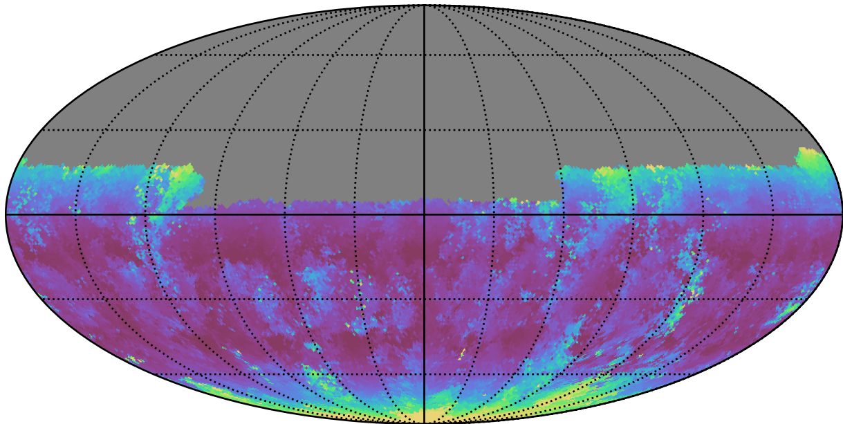
too_elab_r256_d2_gz_v3.4_10yrs Yr 1 u band: Median airmass
