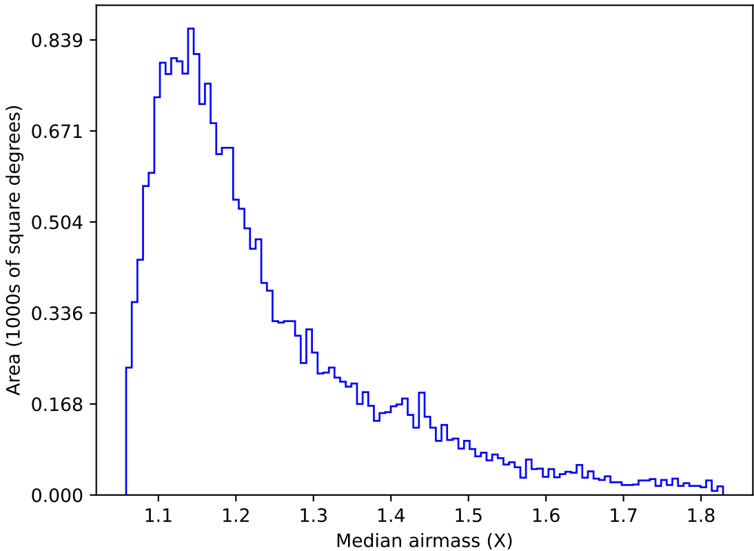
too_elab_r256_d2_gz_v3.4_10yrs Yr 1 u band: Median airmass
