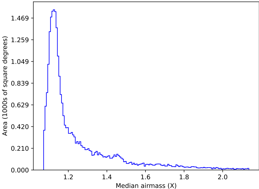
too_elab_r256_d2_gz_v3.4_10yrs Yr 1 all bands: Median airmass
