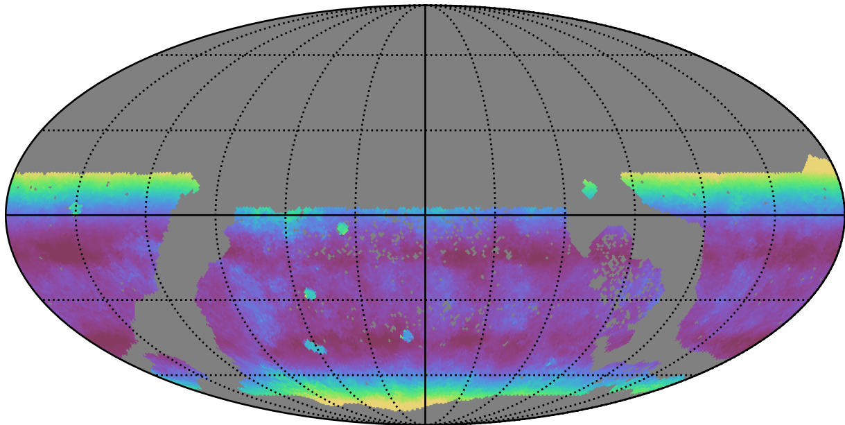
too_elab_r256_d2_gz_v3.4_10yrs WFD z band: Median airmass
