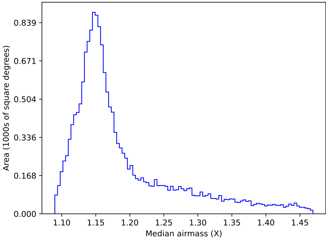
too_elab_r256_d2_gz_v3.4_10yrs WFD z band: Median airmass
