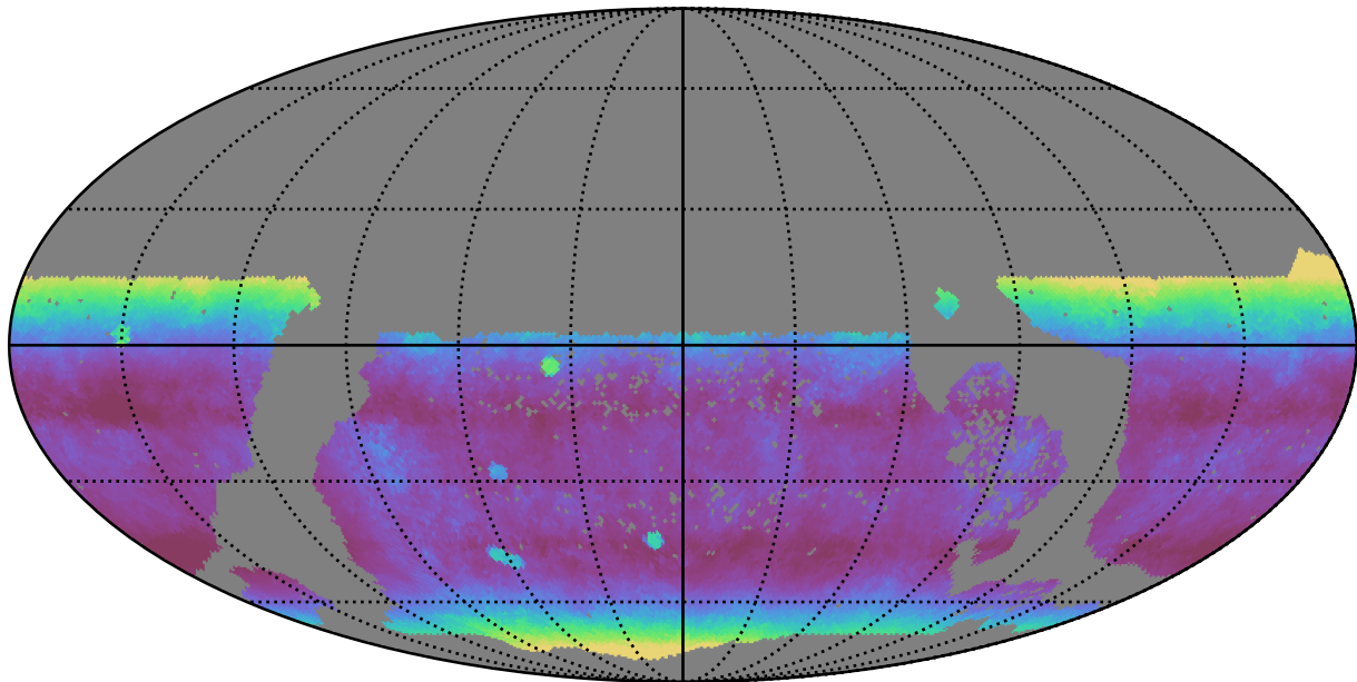
too_elab_r256_d2_gz_v3.4_10yrs WFD y band: Median airmass
