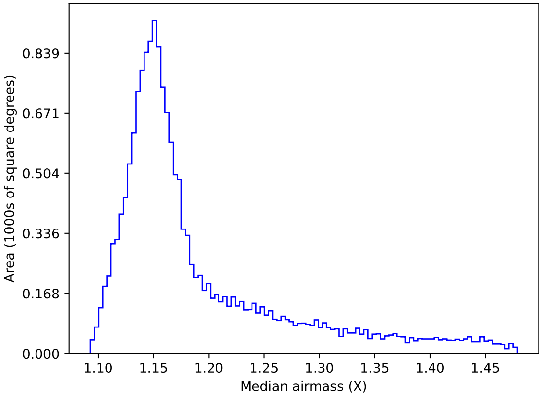
too_elab_r256_d2_gz_v3.4_10yrs WFD y band: Median airmass
