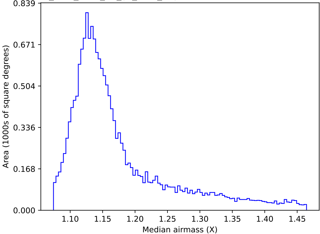
too_elab_r256_d2_gz_v3.4_10yrs WFD r band: Median airmass
