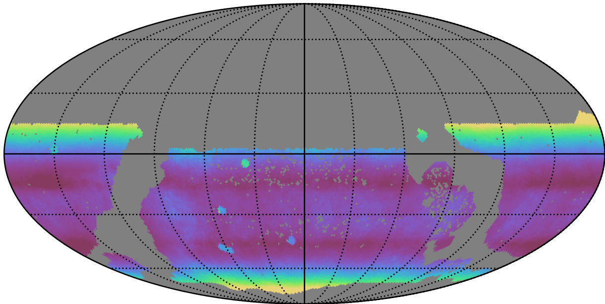
too_elab_r256_d2_gz_v3.4_10yrs WFD all bands: Median airmass
