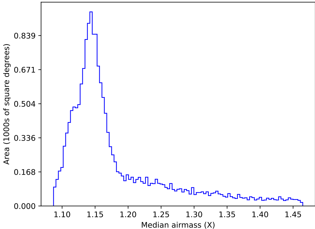
too_elab_r256_d2_gz_v3.4_10yrs WFD all bands: Median airmass
