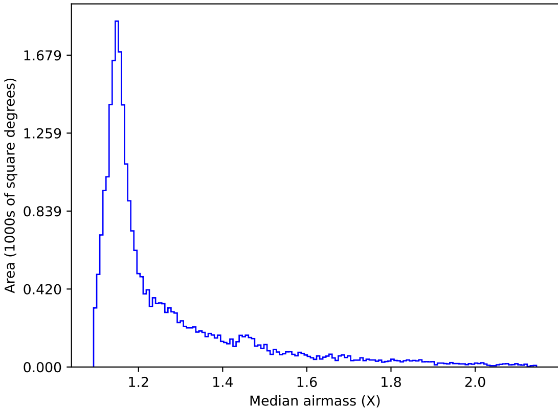
too_elab_r256_d2_gz_v3.4_10yrs All sky z band: Median airmass
