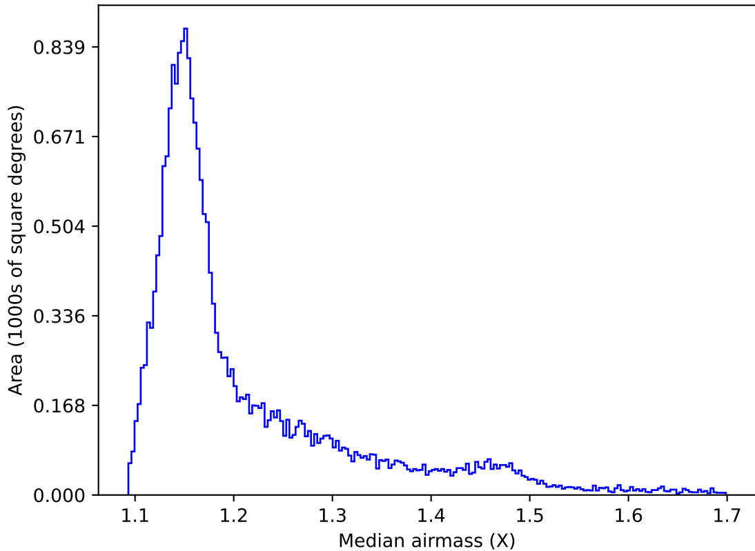
too_elab_r256_d2_gz_v3.4_10yrs All sky y band: Median airmass
