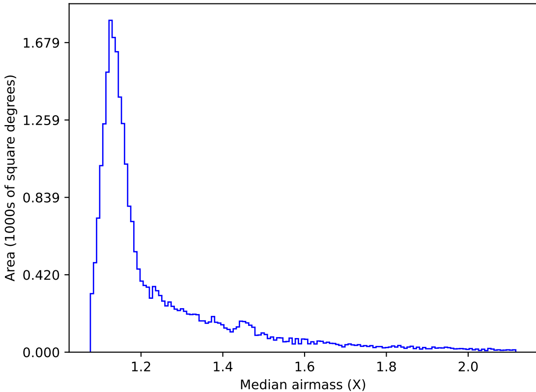
too_elab_r256_d2_gz_v3.4_10yrs All sky r band: Median airmass
