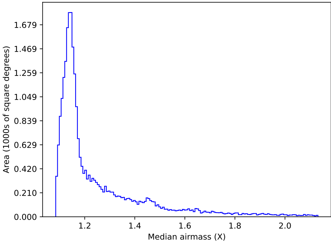
too_elab_r256_d2_gz_v3.4_10yrs All sky i band: Median airmass
